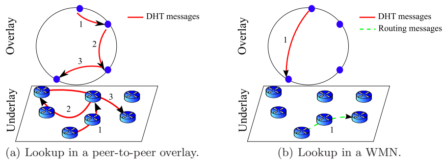
Fig. 1. DHT functionality in two different contexts. Note that in the WMN case, the system relies on an underlying routing protocol running in the backbone.
