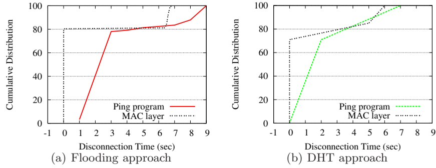
Fig. 10. Cumulative distribution function of disconnection time during handover of the ICMP sender.
