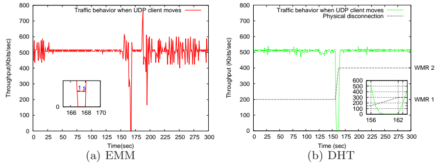
Fig. 7. Disconnection time during the handover of a UDP client.
