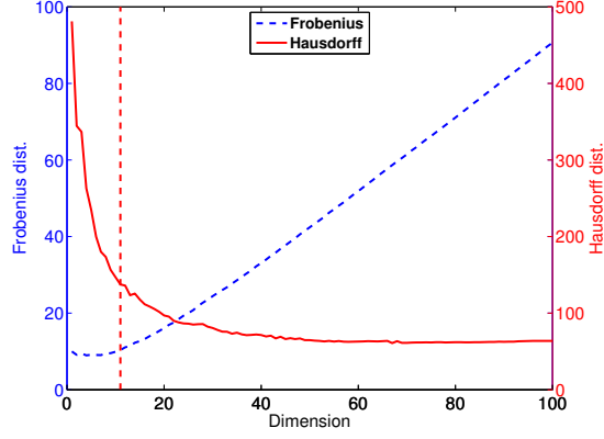
Figure B.7: Scenario 1: \mathcal{X} = \mathbb{R} , variable (mean, variance). Performance of KCP with kernel k^{\text{lin}} . Average distance ( d_F or d_H ) between \hat{\tau}(D) and \tau^* , as a function of D .
