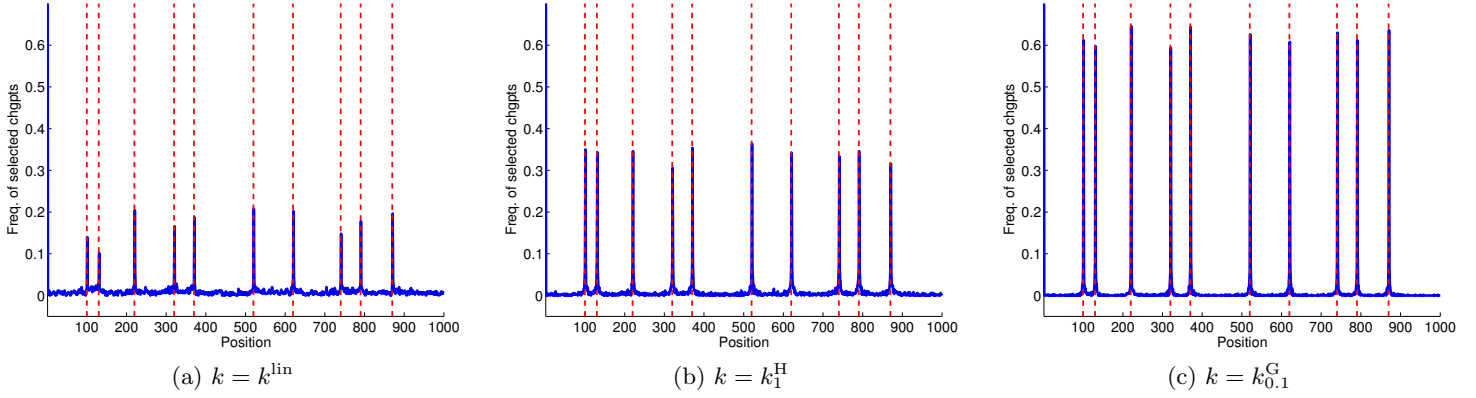
Figure B.9: Scenario 1: \mathcal{X} = \mathbb{R} , variable (mean, variance). Performance of KCP with three different kernels. Probability, for each instant i \in \{1, \dots, n\} , that \hat{\tau}(D^*) puts a change-point at i .
