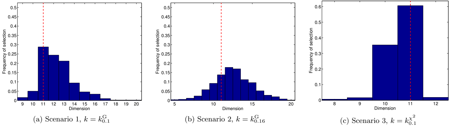
Figure B.14: KCP with a linear penalty (see Section 6.3): distribution of \hat{D} .
