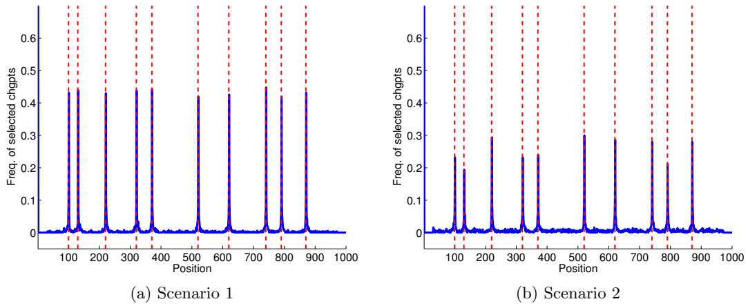
Figure B.18: E-divisive procedure (ED, see Section 6.3) with \alpha = 1 and D = D^* = 11 known: Probability, for each instant i \in \{1, \dots, n\} , that \hat{\tau}_{\text{ED}}(D^*) puts a change-point at i .
