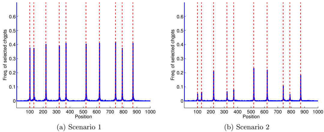
Figure B.17: E-divisive procedure (ED, see Section 6.3) with type-I error level \text{sig.lvl} = 0.05 , \alpha = 1 , and R = 199 : Probability, for each instant i \in \{1, \dots, n\} , that \widehat{\tau}_{\text{ED}} puts a change-point at i .
