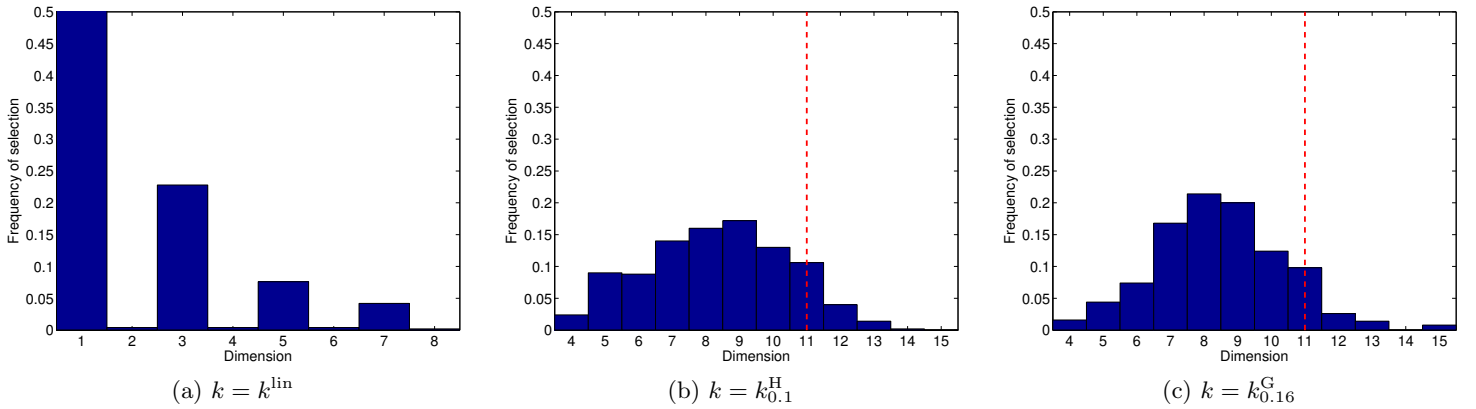
Figure B.12: Scenario 2: \mathcal{X} = \mathbb{R} , constant mean and variance. KCP with three different kernels k . Distribution of \hat{D} .
