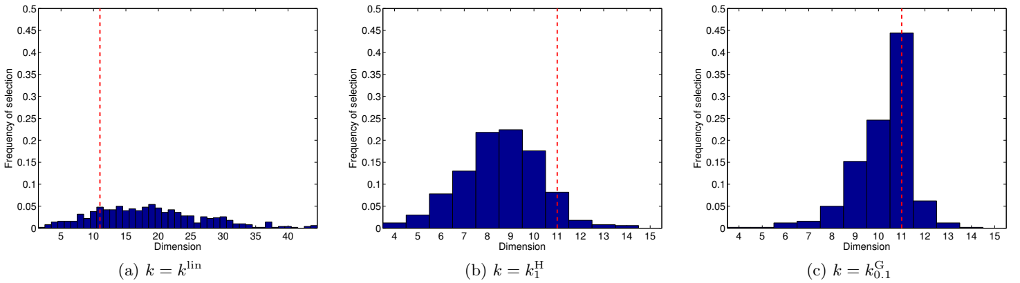
Figure B.8: Scenario 1: \mathcal{X} = \mathbb{R} , variable (mean, variance). KCP with three different kernels k . Distribution of \hat{D} . (Figure B.8c is a copy of Figure 2c, that we repeat here for making comparisons easier.)
