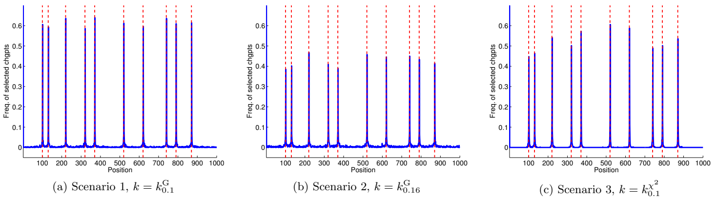
Figure B.15: KCP with a linear penalty (see Section 6.3): Probability, for each instant i \in \{1, \dots, n\} , that \hat{\tau} = \hat{\tau}(\hat{D}) puts a change-point at i .
