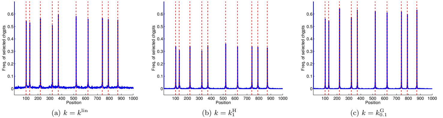
Figure B.10: Scenario 1: \mathcal{X} = \mathbb{R} , variable (mean, variance). Performance of KCP with three different kernels. Probability, for each instant i \in \{1, \dots, n\} , that \hat{\tau} = \hat{\tau}(\hat{D}) puts a change-point at i .
