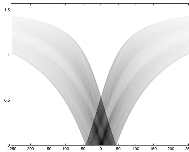
Figure 23. The TV transform of the Shepp-Logan image shown in Figure 19 with d\omega = 0.0025 rad.
