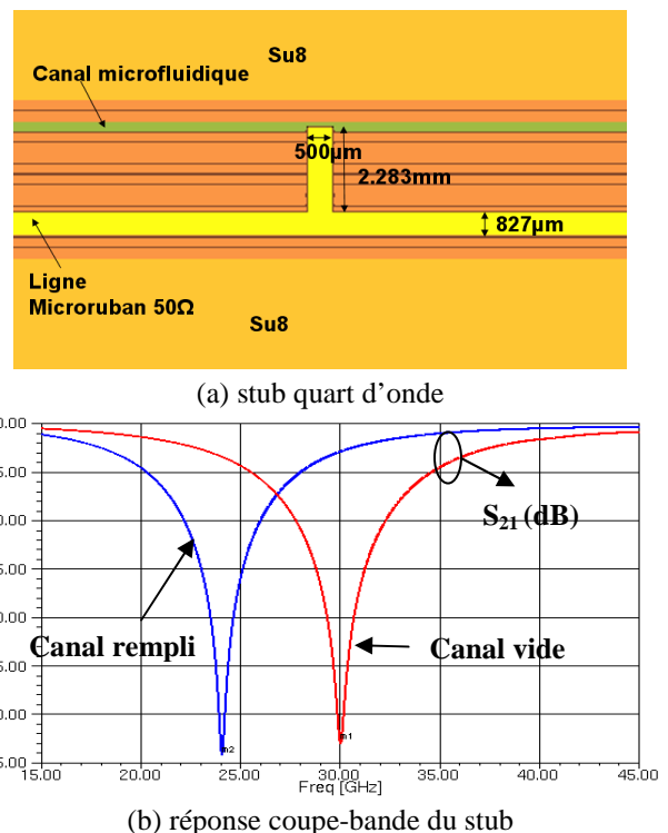
Figure 1. Stub coupe-bande \lambda_g/4
