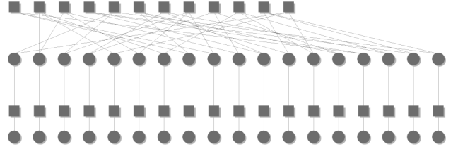
Fig. 2. An example of C_2 . A nonbinary (2,3)-regular LDPC code over \text{GF}(2^m) concatenated with inner multiplicative repetition codes of length 2. The code length is 36 symbols or equivalently 36 m bits. The rate is 1/6.
