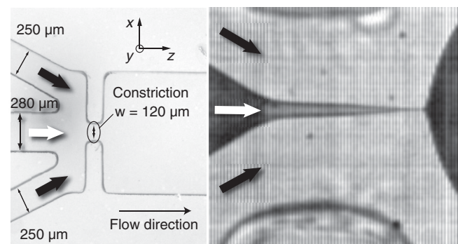
FIG. 1. Schematic of the microfluidic chip. The water solutions are injected along the two side channels (black arrows); the liquid crystal is injected via the middle channel (white arrow). The height of the channel (in the y direction) is 150 \mu\text{m} . The photo shows the rupture of a drop.
