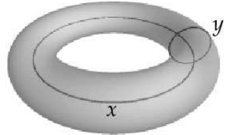
FIGURE 2. Cell structure of the 2–torus
