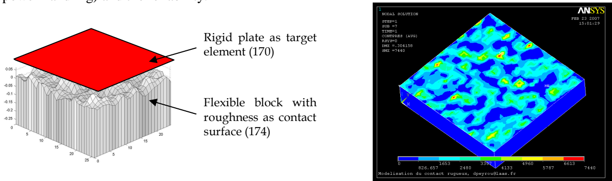
Figure 7: a) The regenerated model in ANSYS for contact resistance simulation. b) Simulation results.
