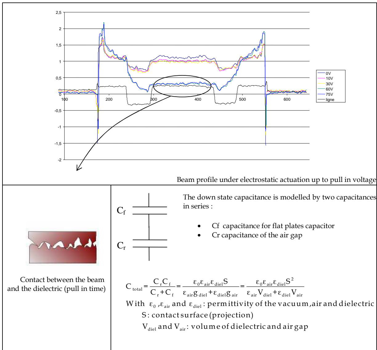
Figure 5: in the top figure we show the switch in contact with the dielectric and below is the model.
