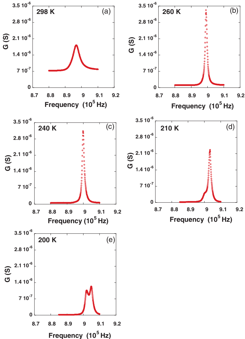
FIG. 2. (Color online) [(a)–(e)] Conductance G vs frequency in transverse mode along [100] from 298 to 200 K for KTP bar samples. When decreasing the temperature the base of conductance is shifted toward low value and at 210 K a small shoulder is visible, moving with temperature and developing into clear splitting of the piezoresonance at 200 K.
