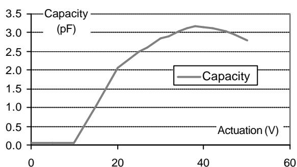
Figure 6 : Capacitance curve, for a maximal theoretical capacitance of 3.6pF
