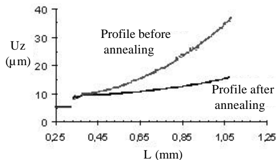
Figure 5: Stress release annealing effect
