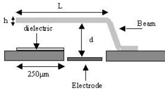
Figure 1: Design geometry
