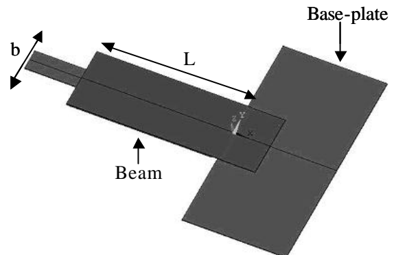
Figure 2: Design top view
