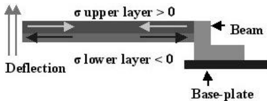
Figure 4: Deflection dues to bi-layer stresses in the beam
