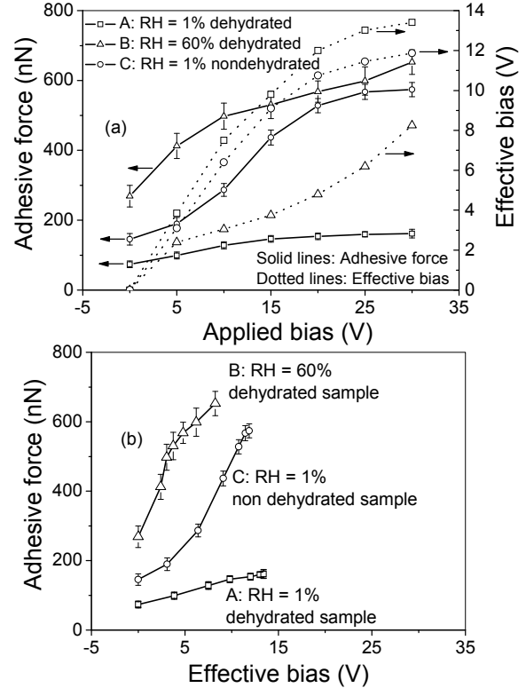
Figure 4. The impact of applied bias on adhesive force.
