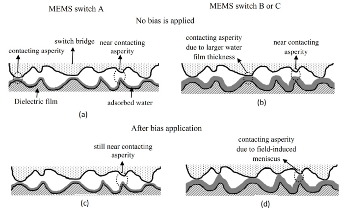
Figure 6. A cartoon showing the meniscus formation at the interface between the switch bridge and the dielectric film for MEMS switches.
