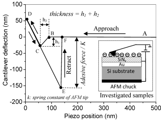
Figure 1. Force-distance curve for the investigated samples.
