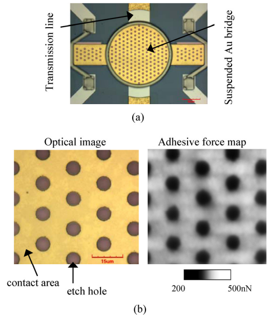
Figure 3. Adhesive force map obtained using the force-distance curve technique for a charged dielectric film implemented in MEMS switch.
