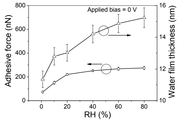
Figure 2. The influence of the relative humidity on adhesive force and adsorbed water film thickness.
