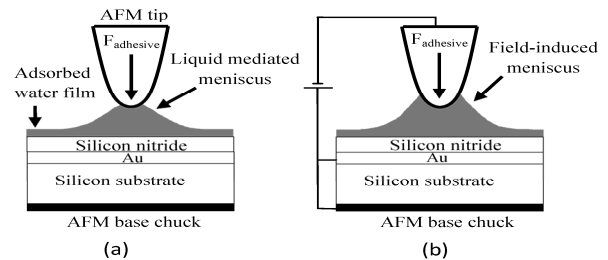
Figure 5. Different mechanisms of meniscus formation between the AFM tip and the sample surface.
