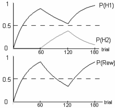
Fig. 2: Conditioning experiment: during the first 60 trials a stimulus event occurs and after 3 seconds a reward is presented. The probability of reward after that stimulus is equal to P(H_1) . Then during the next 60 trials, the stimulus is still presented but not the reward. The probability of reward after that stimulus
