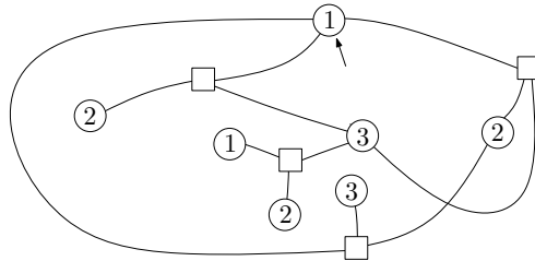
FIGURE 4. A rooted 3-constellation of size 4 (the root corner is pointed with an arrow). This 3-constellation has genus 1 and is unicellular.
