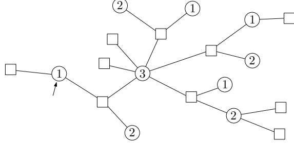
FIGURE 5. A prickly planar 3-quasi-constellation of size n = 6 , with l_1 = 4 , l_2 = 4 , l_3 = 1 . The prickling number is g_0 = 2 .
