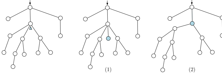
FIGURE 3. Rémy's procedure gives two ways to obtain a plane tree with n edges and a marked vertex v from a plane tree with n-1 edges and a marked corner: (1) in the first way v is a leaf, (2) in the second way v is a non-leaf.
