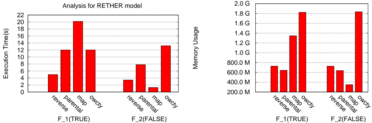
Figure 37: Results for Rether model.
