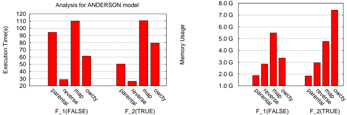
Figure 35: Results for Anderson model.
