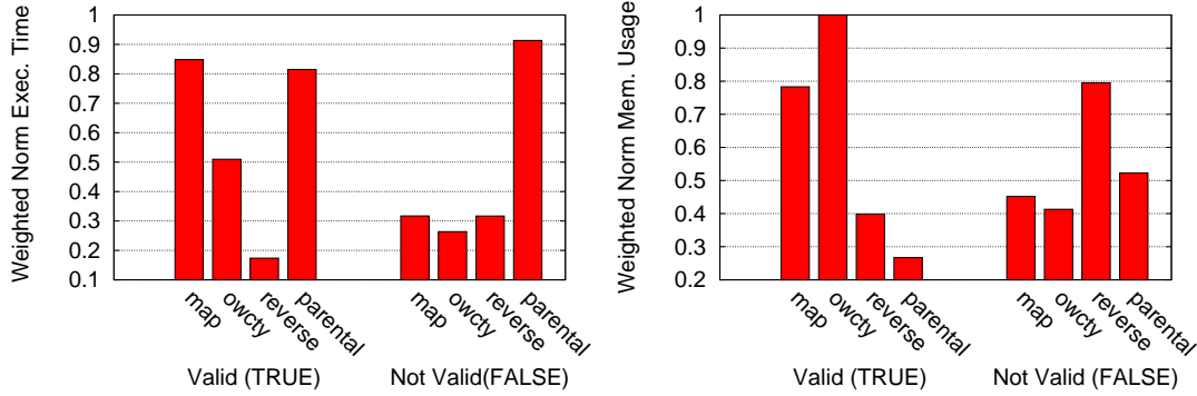
Figure 34: Comparison with divine.
