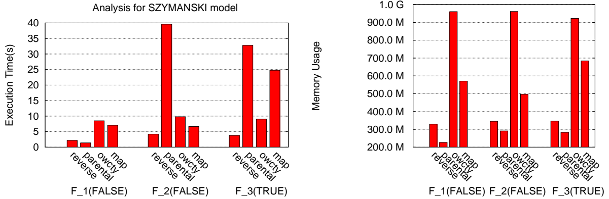
Figure 38: Results for Szymanski model.
