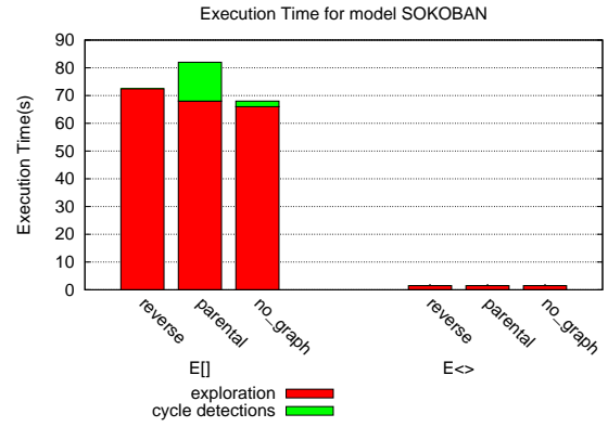
Figure 27: SK model.
