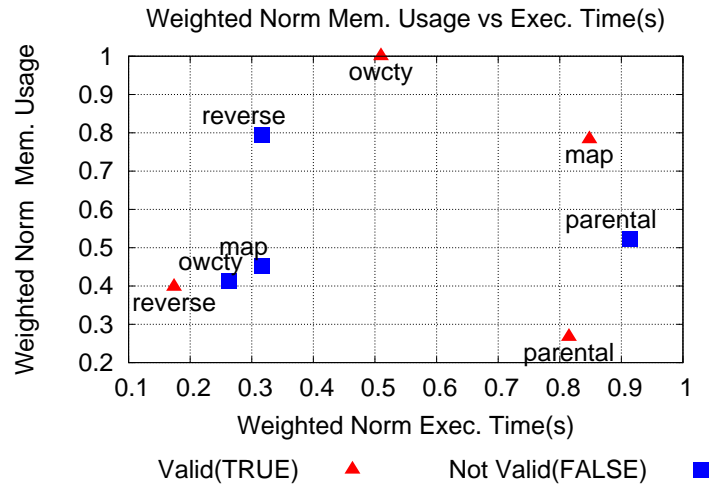
Figure 32: Comparison with divine.
