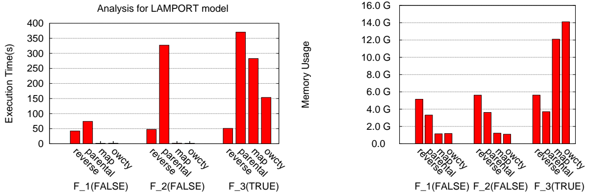
Figure 36: Results for Lamport model.
