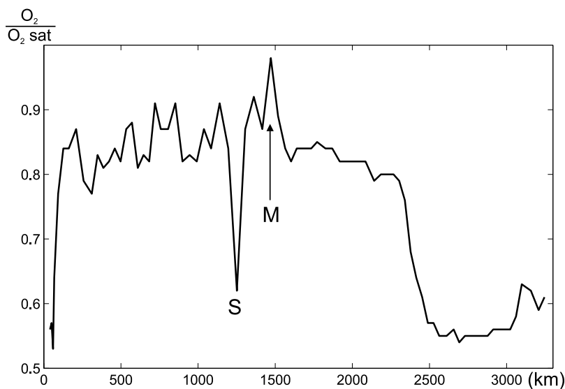
Figure 8. Dissolved oxygen saturations at 300 dbar along the track of the BGH line. The locations of eddies M and S are indicated.
