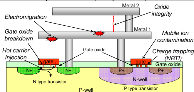
Fig. 1. Common failure mechanisms in CMOS circuits [12]
