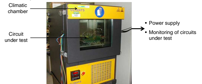
Fig. 9. Climatic chamber for accelerated-life tests
