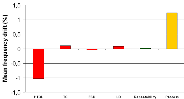
Fig. 16. Spectrum harmonic frequency drifts after various reliability tests
