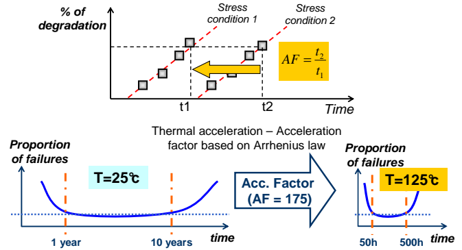
Fig. 2. Principles of accelerated life test
