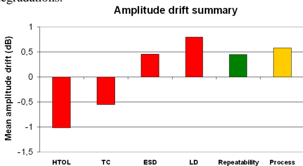
Fig. 15. Emission spectrum mean amplitude drifts after various reliability tests
