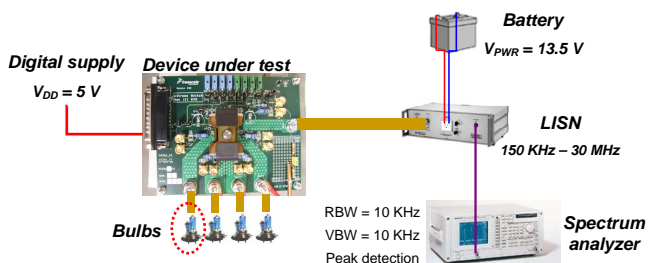
Fig. 10. Power supply conducted emission measurement test-bench
