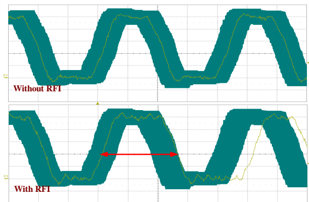
Fig. 7. PLL output signal without (on the left) and with RF injection
