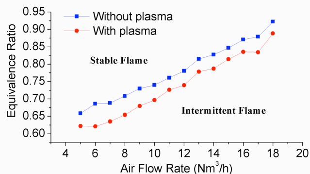
Fig. 3. Flammability limit with NRP plasma in spark regime
