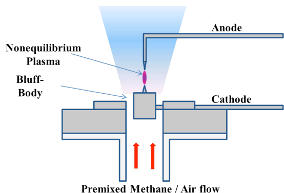
Fig. 2. Experimental setup with premixed burner diagram. The cathode is grounded.
