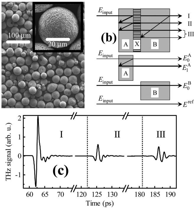
FIG. 1. (a) Scanning electron microscope images of the fabricated TiO 2 microspheres before the sorting procedure. (b) Scheme of the pulse propagation through the structure AXB (sapphire–powder–sapphire) and within the three associated reference measurements. The reflected beams are shifted vertically for graphical clarity. (c) Example of the time-domain signal transmitted through the structure AXB. Dotted lines delimit the intervals containing: I—main pulse ( E_0^{AXB} ); II—1st echo in A ( E_1^{AXB} ); III—superposition of 1st echo in B and 2nd echo in A.
