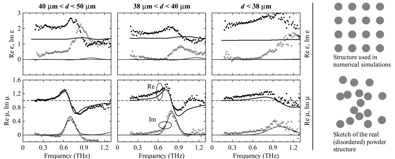
FIG. 2. Permittivity ( \epsilon ) and permeability ( \mu ) of the investigated films. Symbols: measured data; lines: results of numerical simulations with parameters from Table I. Real part: solid line and closed symbols; imaginary part: dotted line and open symbols. Right panel: top—square lattice of TiO 2 microspheres used in numerical simulations; bottom—disordered structure of the powder used in experiments.
