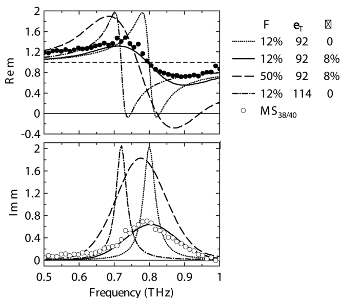
FIG. 3. Lines: calculated permeability of a single layer of monodisperse microspheres with diameter 39 \mu\text{m} . F : filling factor; \epsilon_T : permittivity of the microparticles; P : polydispersity. Symbols: measured permeability of the MS 38/40 sample.
