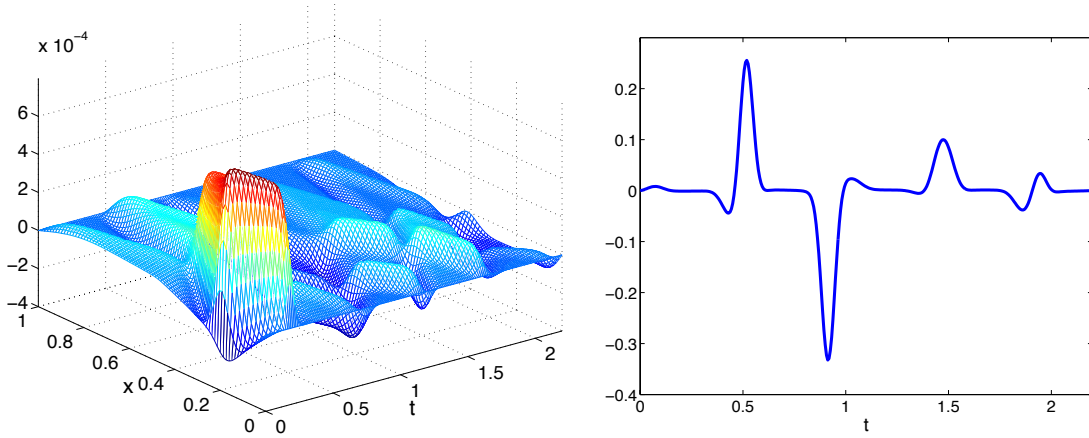
Figure 9: (y_0(x), y_1(x)) \equiv (e^{-500(x-0.2)^2}, 0) and a given by (47) - The solution \hat{p}_h over Q_T (Left) and the corresponding variable \hat{v}_h on (0, T) (Right) - h = (1/80, 1/80) .
