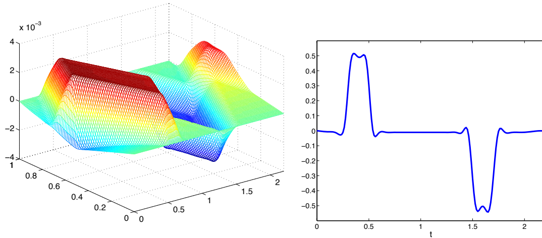
Figure 8: (y_0, y_1) given by (46) and a \equiv 1 - The solution \hat{p}_h over Q_T ( Left ) and the corresponding variable \hat{v}_h on (0, T) ( Right ) - h = (1/80, 1/80) .
