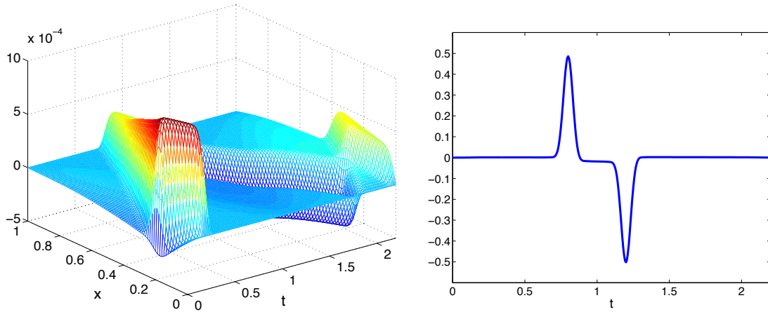
Figure 4: (y_0(x), y_1(x)) \equiv (e^{-500(x-0.2)^2}, 0) and a \equiv 1 - The solution \hat{p}_h over Q_T ( Left ) and the corresponding variable \hat{v}_h on (0, T) ( Right ) - h = (1/80, 1/80) .
