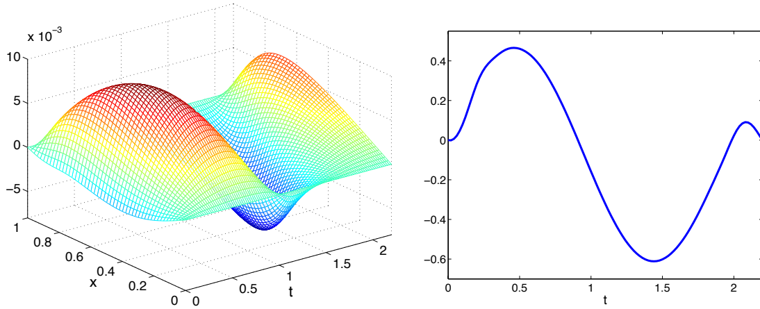
Figure 2: (y_0(x), y_1(x)) \equiv (\sin(\pi x), 0) and a \equiv 1 - The solution \hat{p}_h over Q_T ( Left ) and the corresponding variable \hat{v}_h on (0, T) ( Right ) - h = (1/80, 1/80) .
