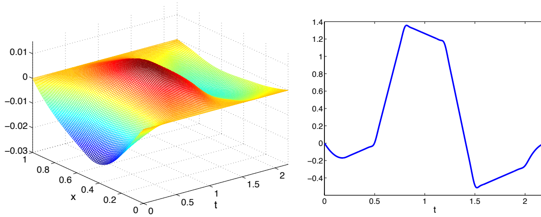
Figure 6: (y_0, y_1) given by (45) and a \equiv 1 - The solution \hat{p}_h over Q_T ( Left ) and the corresponding variable \hat{v}_h on (0, T) ( Right ) - h = (1/80, 1/80) .
