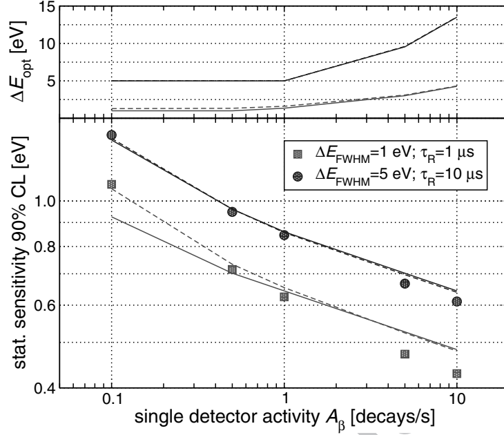
Figure 2: Comparison between the statistical sensitivity as estimated by a Montecarlo approach (symbols) and by the analytic formulation (lines). The continuous and dashed lines are obtained using (14) with (15) and (16) respectively. The statistical sensitivity is evaluated for an exposure T = 10000 detector \times year. The rightmost point corresponds to a total statistics N_{ev} = 3 \times 10^{12} . The upper panel shows how \Delta E_{opt} gets larger as the pile-up spectrum increase its weight.
