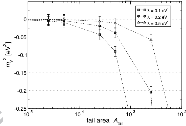
Figure 14: Systematic effect caused on m_\nu^2 by an undetected exponential tail in a Gaussian response function R(E) . The Montecarlo parameters are N_{ev} = 10^4 , \Delta E_{FWHM} = 1.5 eV, f_{pp} = 10^{-6} and bT = 0 c/eV.
