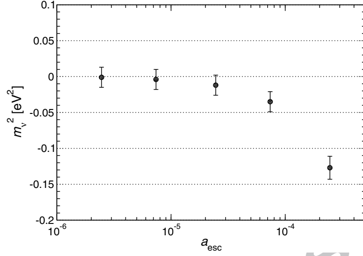
Figure 7: Systematic m_v^2 shift caused by ignoring the correction for the surface electron escape. Points obtained for N_{ev} = 10^{14} , \Delta E_{FWHM} = 1.5 eV, f_{pp} = 10^{-6} and bT = 0 c/eV.
