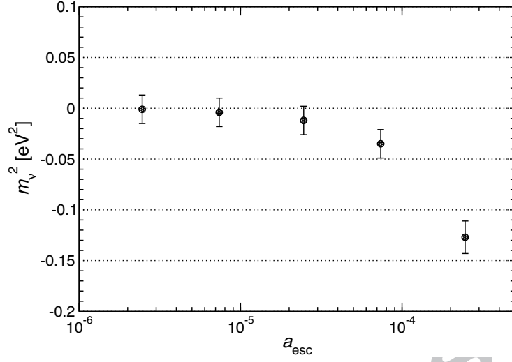
Figure 7: Systematic m_v^2 shift caused by ignoring the correction for the surface electron escape. Points obtained for N_{ev} = 10^{14} , \Delta E_{\text{FWHM}} = 1.5 eV, f_{pp} = 10^{-6} and bT = 0 c/eV.
