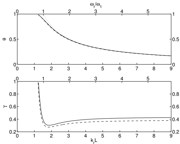
Figure 4: Comparison of the first regime for L=57\text{cm} (—) and L=14.69\text{cm} (---). Lower plot: dimensionless blowing pressure \gamma of the bifurcation. Upper plot: corresponding dimensionless frequency ratio \theta = \omega/\omega_r ; the first passive resonance of the bore is reminded ( \cdots ).
