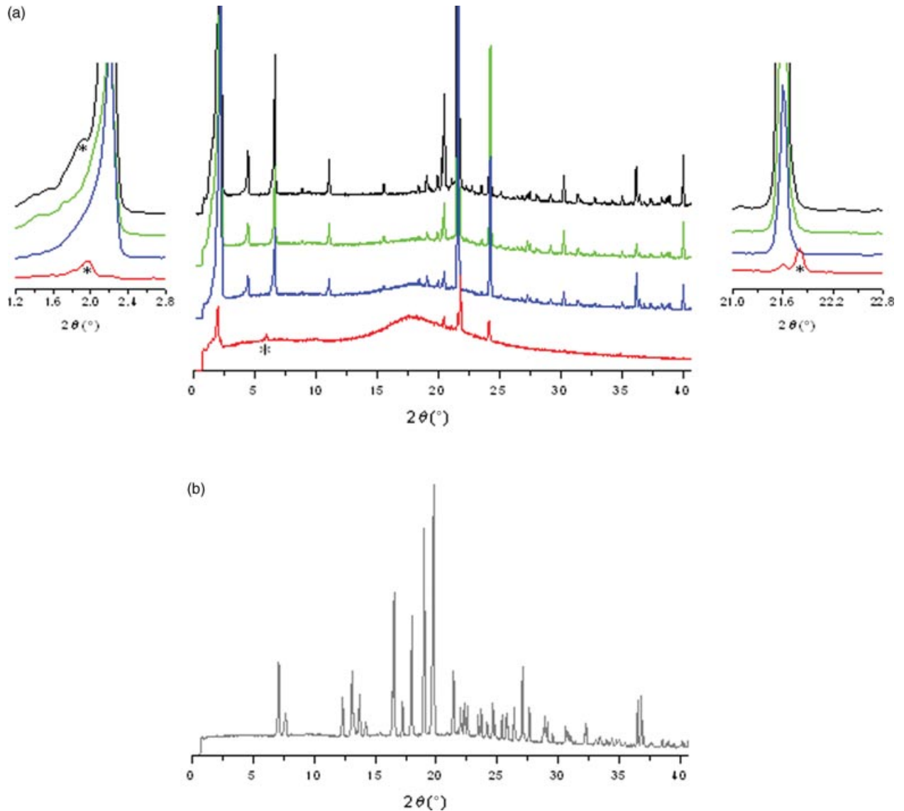
Figure 8. Experimental XRPD of (a) selected S-ibuprofen/stearic acid mixtures and (b) pure S-ibuprofen. The patterns were shifted for clarity. (a) S-ibuprofen molar ratios: 0.000 (black), 0.334 (green), 0.501 (blue), and 0.929 (red). The samples were analyzed 3 days after being melted at 80°C directly in the capillary, and then annealed at room temperature. (Insets) Corresponding patterns focused between 1.2° and 2.8° (left) and between 20.8° and 22.8° (right). The * indicates the signal corresponding to the stearic acid E_m -form.
