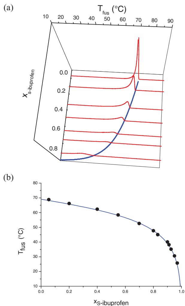
Figure 6. (a) Three-dimensional representation of selected DSC thermograms (red curves) obtained for the S-ibuprofen/stearic acid mixtures and recorded upon heating after cooling from the molten state. Endothermic transformations give signals pointing up. (b) The corresponding T - x phase diagram. The liquidus curve is represented in blue.
