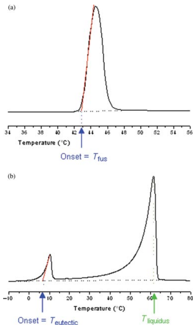
Figure 2. DSC thermogram examples obtained for (a) a pure compound and (b) a binary eutectic mixture. The corresponding temperature assignments are indicated. Endothermic transformations give signals pointing up.
