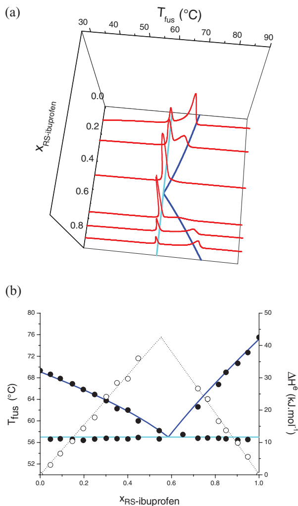
Figure 4. (a) Three-dimensional representation of selected DSC thermograms obtained for the RS-ibuprofen/stearic acid mixtures (red curves). Endothermic transformations give signals pointing up. (b) The corresponding T - x phase diagram (left axis). The Tammann plot is represented by the open circles and dotted lines (right axis). The eutectic and liquidus curves are represented in cyan and blue, respectively.
