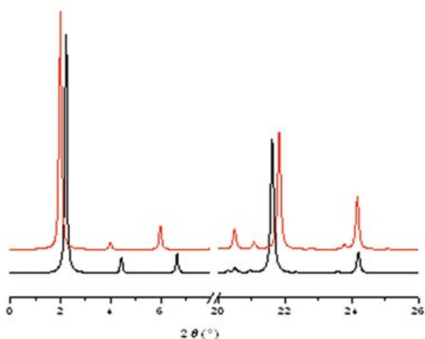
Figure 9. Calculated XRPD patterns of C- (black) and E m - (red) stearic acid polymorphs; from Refs. 13 and 15, respectively. The patterns were shifted for clarity.
