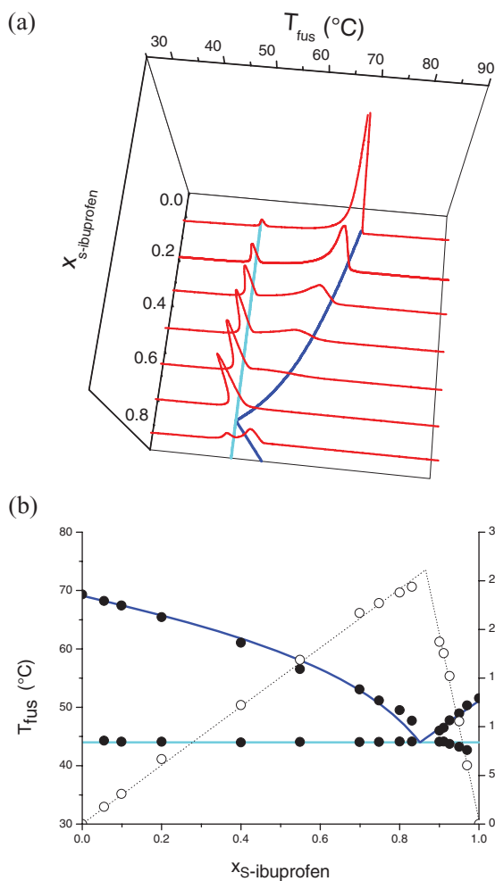
Figure 5. (a) 3D representation of selected DSC thermograms obtained for the S-ibuprofen/stearic acid mixtures (red curves). Endothermic transformations give signals pointing up. (b) The corresponding T - x phase diagram (left axis). The Tammann plot is represented by the open circles and dotted lines (right axis). The eutectic and liquidus curves are represented in cyan and blue, respectively.
