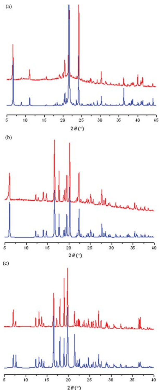
Figure 3. XRPD patterns of (a) stearic acid, (b) RS-ibuprofen, and (c) S-ibuprofen. For a same panel, the upper and lower curves correspond to the experimental and calculated 1,13,21 patterns, respectively.
