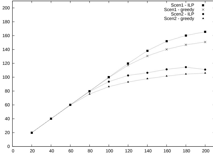
Figure 4: Average numbers of accepted users obtained by the proposed algorithms for each number of users
