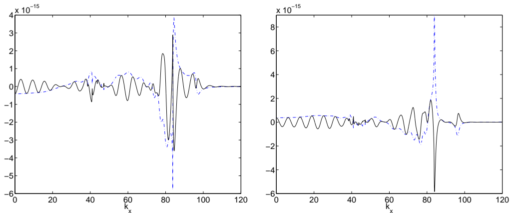
Figure 2: Processing the integrals: real part (left) and imaginary part (right) of \overline{u}_y^*(k_x, \omega_0) (dashed line) and \overline{u}_y^*(k_x, \omega_0) \cos(k_x x) (solid line). This signal is obtained at recorder R_4 in the case of N = 4 interfaces, with sealed pore conditions; see section 5 for details.
