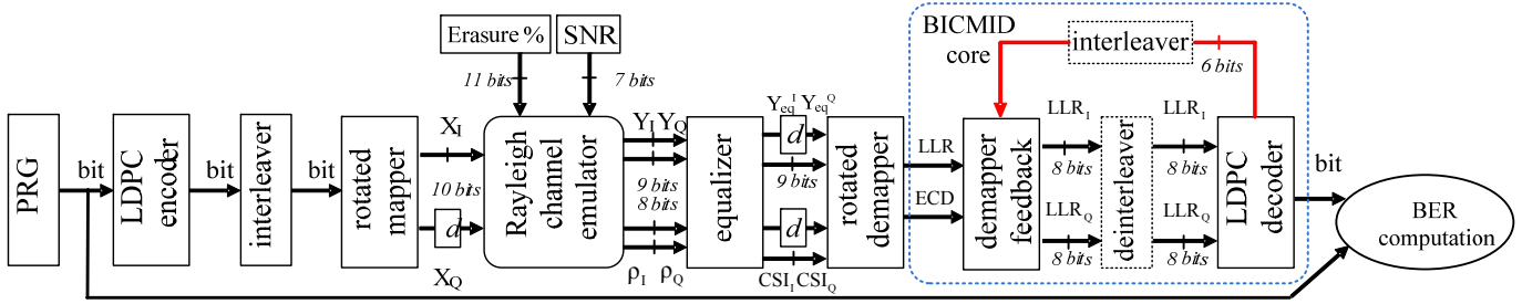
Fig. 8: Experimental setup for prototyping the BICM receiver
