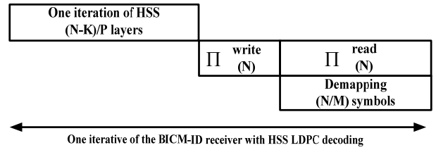
Fig.4. (a) Scheduling of horizontal iterative receiver
