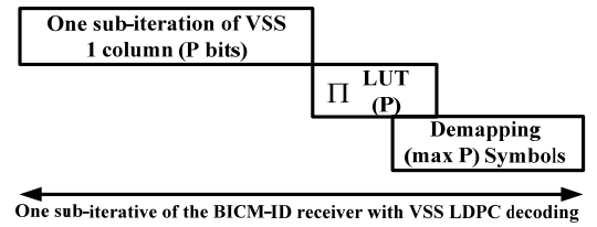
Fig.4. (b) Scheduling of vertical iterative receiver
