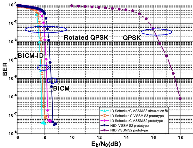
Fig. 9: Performance comparison for QPSK over a fading channel with 15 % of erasures. 64K frames, DVB-T2 LDPC, rate R=4/5
