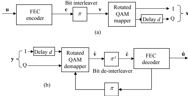
Fig. 1. (a) The BICM with SSD transmitter; (b) Conventional BICM-ID receiver.
