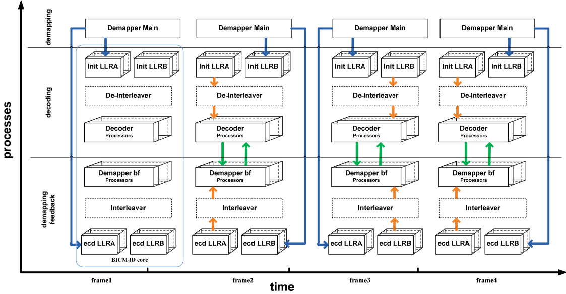
Fig. 5. The proposed architecture of the vertical iterative receiver
