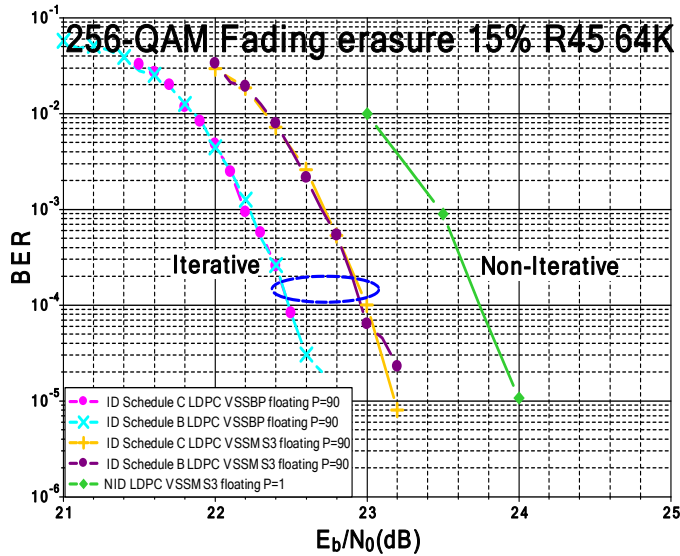
Fig. 3. Performance comparison for rotated 256-QAM over a fading channel with 15% of erasures. DVB-T2 64K LDPC, rate R=4/5
