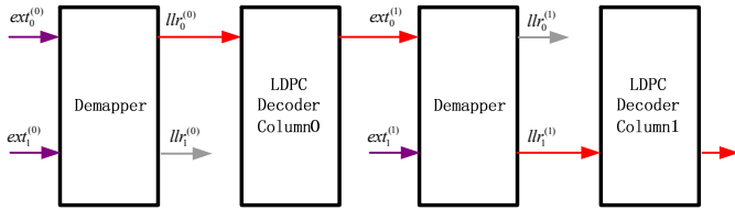
Fig. 6. Efficient message passing schedule for BICM-ID QPSK
