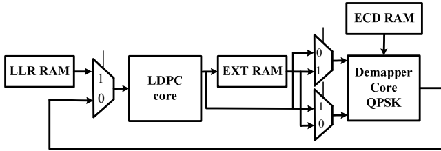
Fig. 7. Selection process for the message exchange in the receiver
