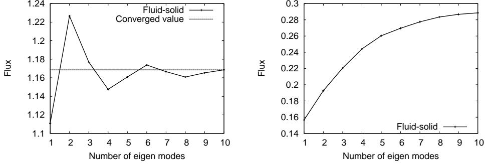
FIGURE 4. Evaluation of \text{Flux}_{\text{fluid/solid}} according to the number of considered eigenmodes for the infinite domain configuration on the left and for the semi infinite one on the right, for both cases Pe = 10 .
