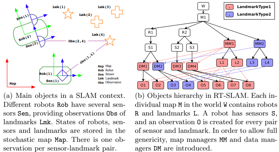
Fig. 1. The main objects in RT-SLAM
