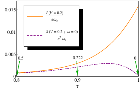
FIG. 3: dc current and ZF noise as a function of the effective transmission \tau , for eV/\hbar\omega_c = 0.2 , at a low temperature: k_B T/\hbar\omega_c = 0.001 . The arrows indicate the associated values of eV_B/\hbar\omega_c . With a frequency cutoff of about 1 THz, the value 0.01 e\omega_c on the axis corresponds to a current of about 10 nA.
