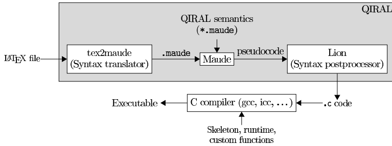
Figure 3: Overview of QIRAL compilation chain
