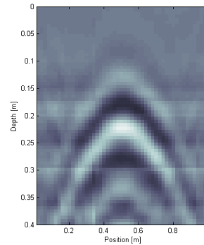
Figure 4 : measurements over a metallic sphere after the clutter effects have been subtracted
