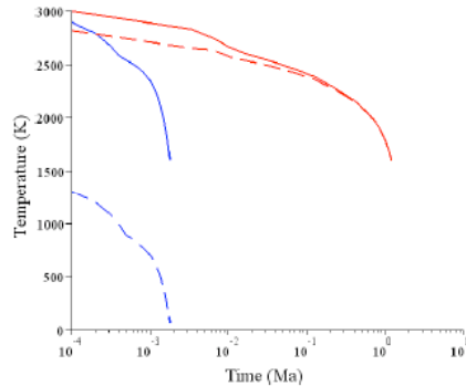
Figure 1: Temporal evolution of potential (Solid line) and surface (Dash line) temperature of the magma ocean with (red line) or without (blue line) interaction with the atmosphere.
