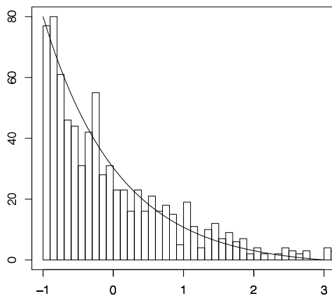
Figure 11: Histogram of the \mathbf{X}'_i 's in the exponential case with n = 1000 and k = 800 for P_n = 10^{-2} . The curve represents the associated tilted density.
