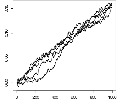
Figure 6: Trajectories in the normal case for P_n = 10^{-8}
