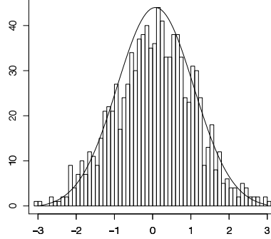
Figure 9: Histogram of the \mathbf{X}'_i 's in the normal case with n = 1000 and k = 999 for P_n = 10^{-2} . The curve represents the associated tilted density.
