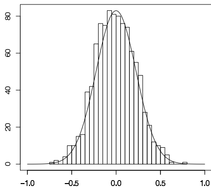
Figure 13: Histogram of the \mathbf{X}'_i 's in the normal case with n = 1000 , k = 800 and u(x) = x^2 for P_n = 10^{-8} . The curve represents the associated tilted density.
