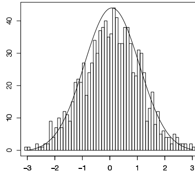
Figure 9: Histogram of the \mathbf{X}'_i 's in the normal case with n = 1000 and k = 999 for P_n = 10^{-2} . The curve represents the associated tilted density.
