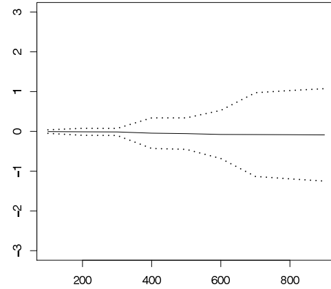
Figure 4: ERE(k) (solid line) along with upper and lower bound of CI(k) (dotted line) as a function of k with n = 1000 and a such that P_n \simeq 10^{-8} .
