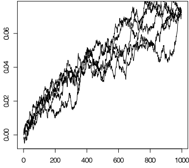
Figure 5: Trajectories in the normal case for P_n = 10^{-2}
