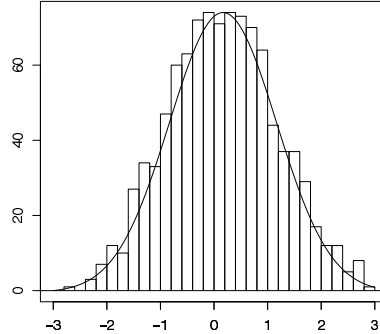
Figure 10: Histogram of the \mathbf{X}'_i 's in the normal case with n = 1000 and k = 999 for P_n = 10^{-8} . The curve represents the associated tilted density.
