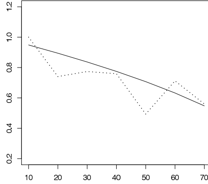
Figure 15: Ratio of the empirical value of the MSE of the adaptive estimate w.r.t. the empirical MSE of the i.i.d. twisted one (dotted line) along with the true value of this ratio (solid line) as a function of k .
