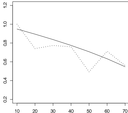
Figure 15: Ratio of the empirical value of the MSE of the adaptive estimate w.r.t. the empirical MSE of the i.i.d. twisted one (dotted line) along with the true value of this ratio (solid line) as a function of k .
