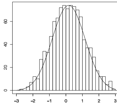
Figure 10: Histogram of the \mathbf{X}'_i 's in the normal case with n = 1000 and k = 999 for P_n = 10^{-8} . The curve represents the associated tilted density.
