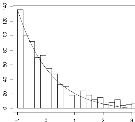
Figure 12: Histogram of the \mathbf{X}'_i 's in the exponential case with n = 1000 and k = 800 for P_n = 10^{-8} . The curve represents the associated tilted density.
