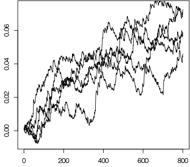
Figure 7: Trajectories in the exponential case for P_n = 10^{-2}
