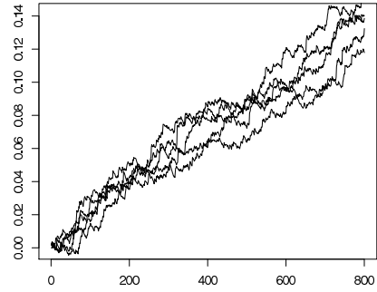
Figure 8: Trajectories in the exponential case for P_n = 10^{-8}
