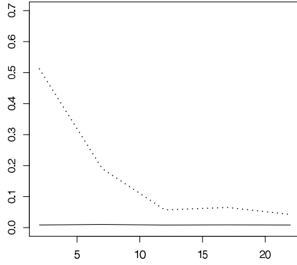
Figure 14: Variance of \widehat{\theta}_k , the initial estimator (dotted line), along with the variance of \theta_{RB,k} , the Rao-Blackwellised estimator (solid line) with n = 100 as a function of k .
