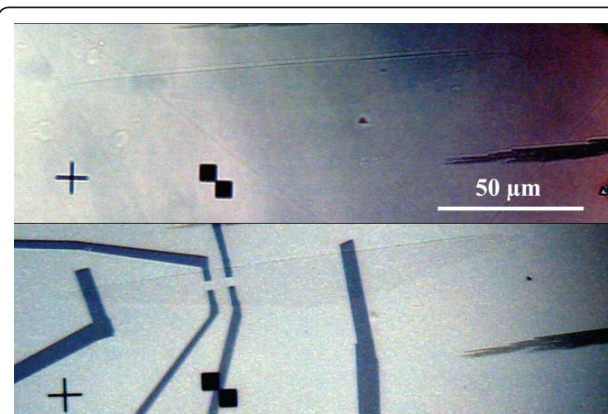
Figure 3 Optical microscopy of a SLEG grown on 8° off-axis semi-insulating SiC substrate. (a) before contact and (b) after contacting in a Hall Bar configuration for Hall Effect measurement.
