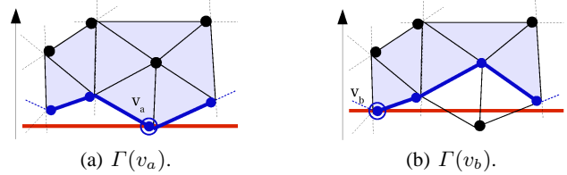
Fig. 7 Example of continuous (red) and discrete (blue) level lines (height function). The upper valued triangulation T^+ is colored in light blue.
