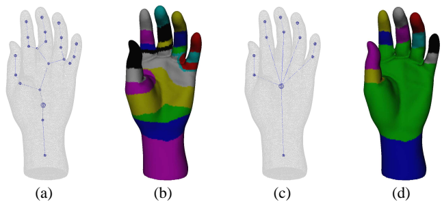
Fig. 19 Topology driven segmentation overview: a raw segmentation (b) is obtained from the enhanced topological skeleton (a), then a node merging algorithm (c) completes the process (d).
