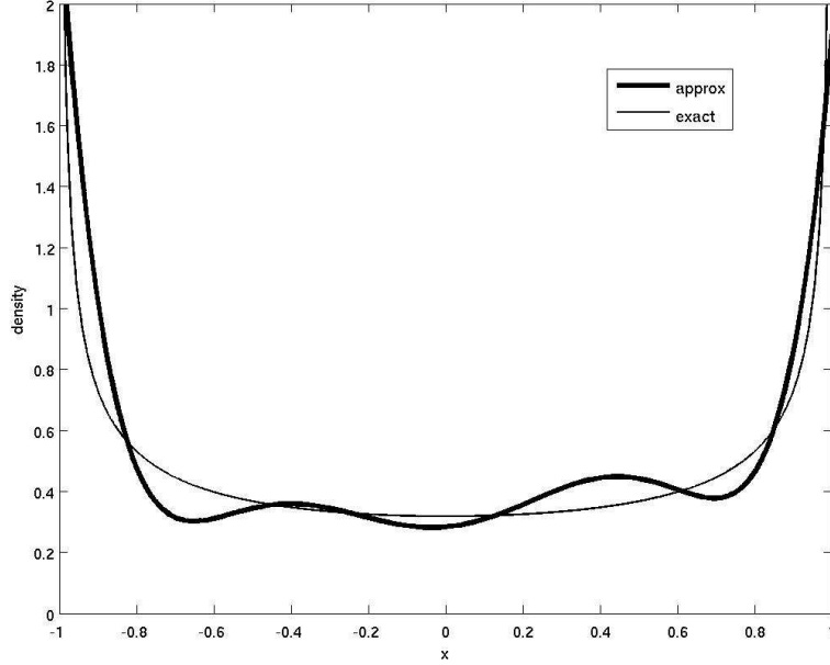
Figure 1: Approximate density (thick) and exact density (thin) of the continuous measure invariant for the logistic map.
