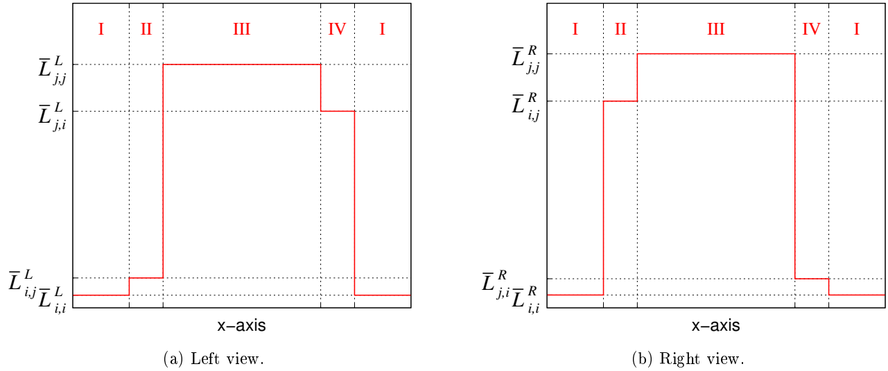
Figure 3: Spatial profiles observed from the left eye position (a) and from the right eye position (b) along the dotted line in Figure 1. Values correspond to the average luminance measured through each glass for each regions of the stereoscopic image (cf. Equation 3).
