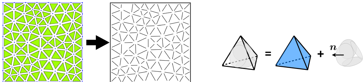
Figure 1: From cohesive-volumetric discretization to the equivalent 'matrix-inclusions' composite.
