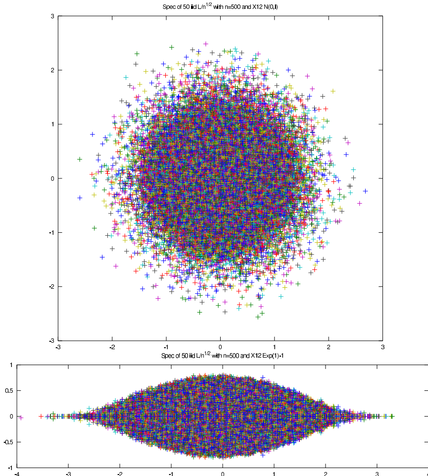
FIGURE 1.1. The bottom graphic shows a simulation of 50 i.i.d. copies of the spectrum of n^{-1/2}L with n = 500 when \mathcal{L} is the exponential law on \mathbb{R} of parameter 1 shifted by -1 ( m = 0 , K_{11} = 1 , and K_{12} = K_{21} = K_{22} = 0 ). The top graphics shows a simulation of 50 i.i.d. copies of the spectrum of n^{-1/2}L with n = 500 when \mathcal{L} is the Gaussian law on \mathbb{C} of mean 0 and covariance K = \frac{1}{2}I_2 . These simulations and graphics were produced with the free software GNU Octave provided by Debian GNU/Linux.
