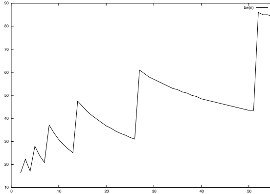
Fig. 2: Function bw(n) for \delta=100 ms and s=2000 bytes.
