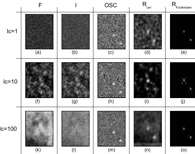
Fig. 5. Detection in scenario 1 corresponding to OSC contrast only. Horizontally: illumination pattern \mathbf{F} , intensity image, OSC, the results of \mathcal{R}_{uni} and \mathcal{R}_{Funknown} detection. Vertically: those images are computed for l_c=1, 10, and 100 .
