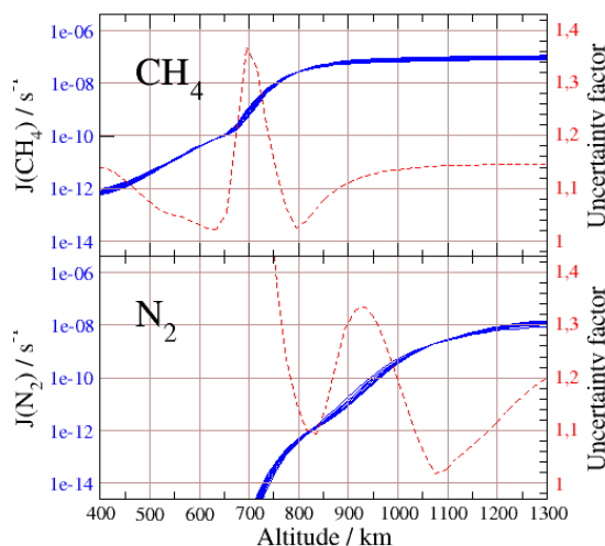
Figure 1: Samples of altitude-dependent photolysis rate coefficients for N_2 and CH_4 (lines; left scale) and their uncertainty factors (dashed lines; right scale).
