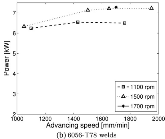
Fig. 17. Variation of the total power P estimated from the torque measurement as a function of the welding parameters.
