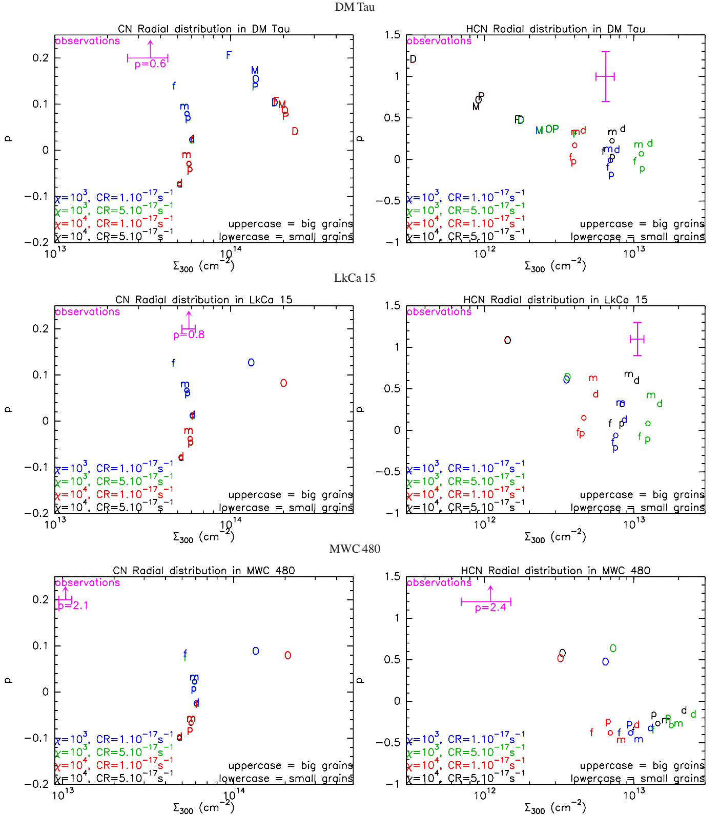
Fig. B.1. Value of \Sigma_{300} and p from our chemistry modeling for the three sources, with our “standard” chemistry. o: density and temperature from theoretical models, p: temperature increased by 30%, m: temperature decreased by 30%, f: density multiplied by a factor 3 and d: density divided by a factor 3. In many models the blue and green markers overlap, as do the red and black ones.
