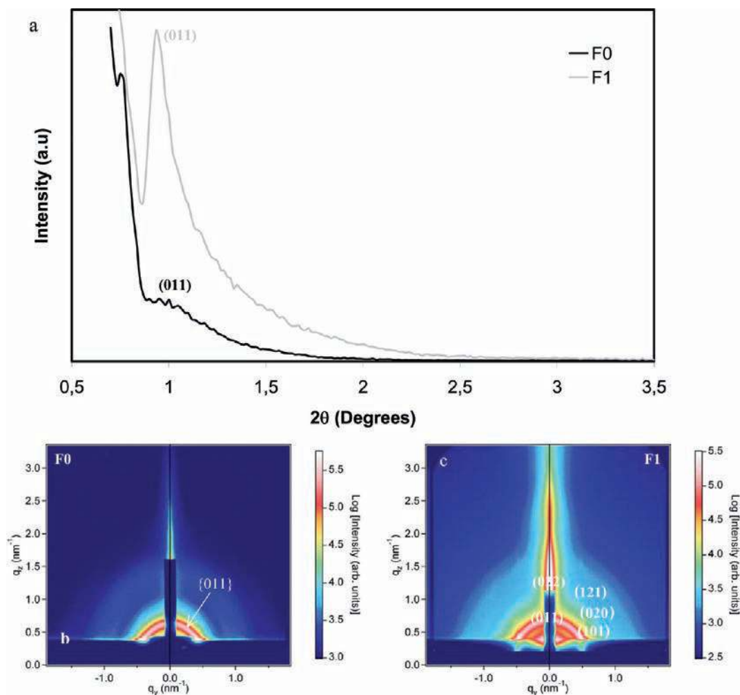
Figure 1. (a) Small-angle XRD patterns of F0 and F1 samples. (b) GISAXS pattern of the F0 sample. (c) GISAXS pattern of the F1 sample (cubic indexation).
