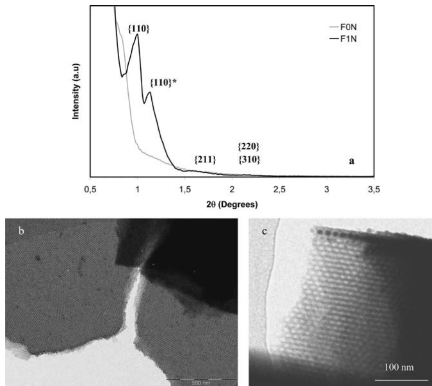
Figure 4. (a) Small-angle XRD pattern of the F1N sample; * probably corresponding to the superficial layers. (b) TEM top view of the F1N sample. (c) TEM cross-section of the F1N sample. Zone axis [11-1] .
