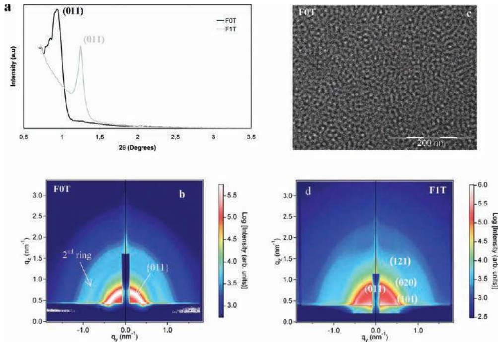
Figure 2. (a) Small-angle XRD patterns of F0T and F1T samples. (b) GISAXS pattern of the F0T sample. (c) TEM top view of the F0T sample. (d) GISAXS pattern of the F1T sample (diffraction spots indexed in Im-3m).
