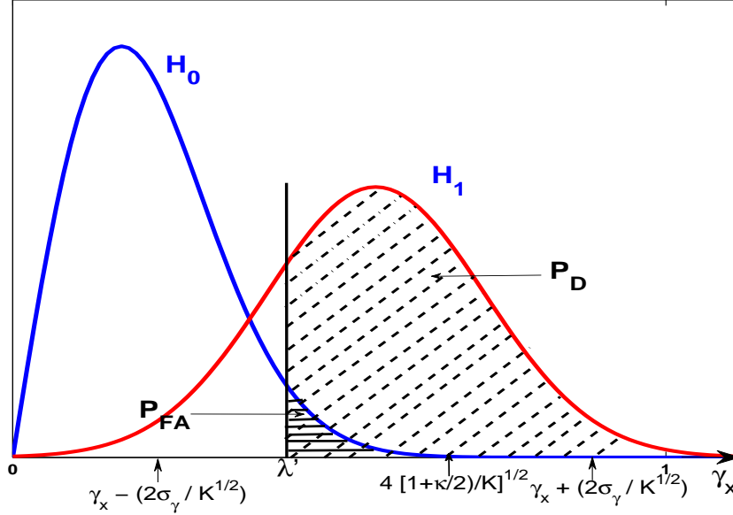
Fig.1 Approximative probability density function (PDF) of \hat{\gamma}_x under H_0 and H_1 .
