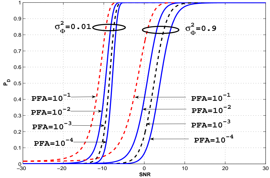
Fig.2 P_D for four different fixed P_{FA} and two values of \sigma_{\phi_1} as a function of SNR for N = Q = 1 and K = 100 .
