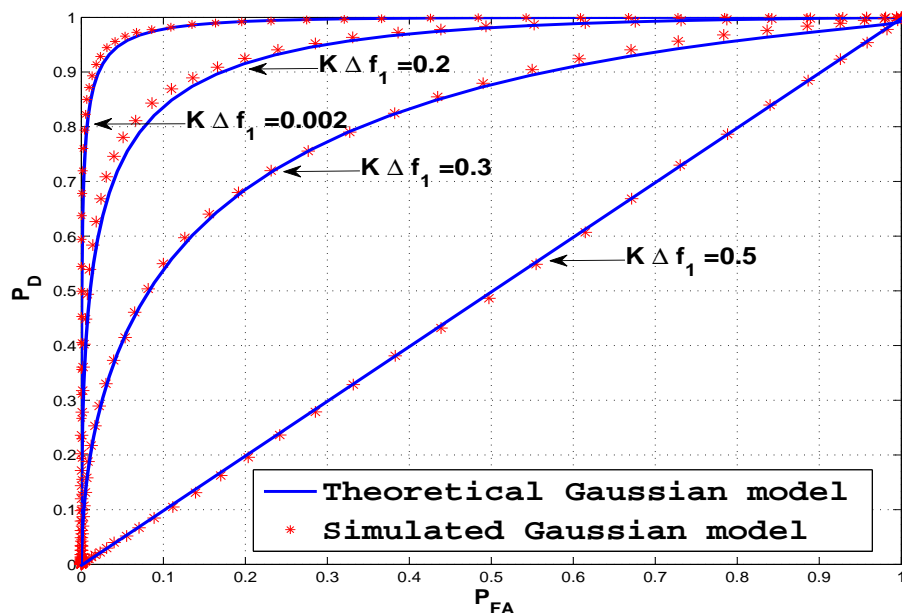
Fig.4 Asymptotic theoretical and empirical (with 10000 Monte Carlo runs) ROC curve associated with Gaussian model for four values of K\Delta f_1 .
