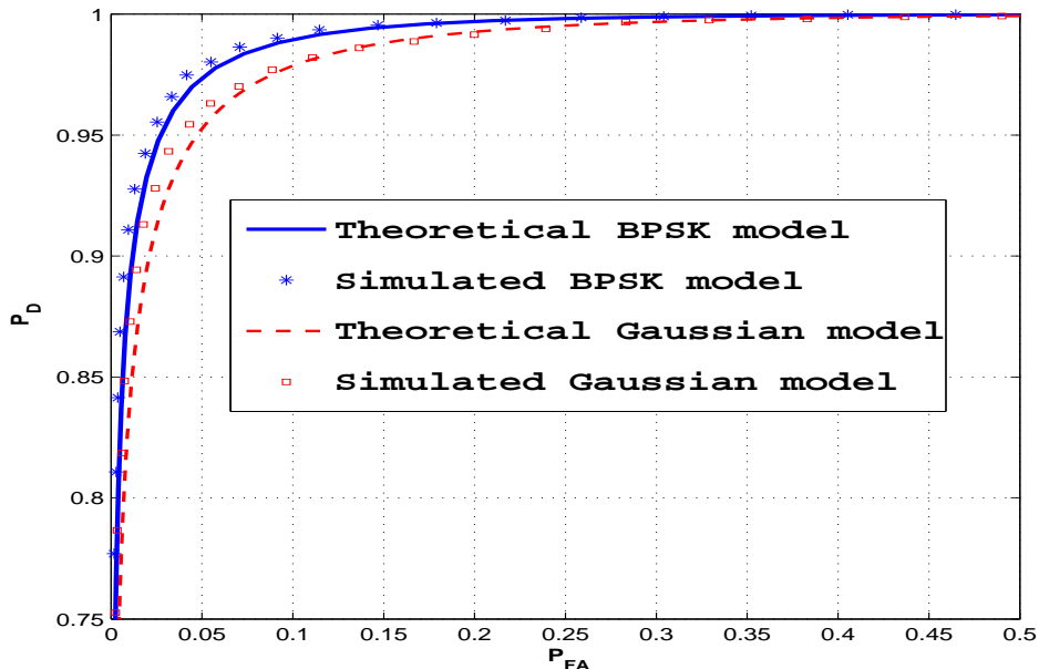
Fig.3 Asymptotic theoretical and empirical (with 10000 Monte Carlo runs) ROC curve associated with BPSK and Gaussian model.
