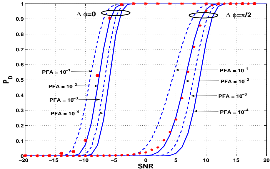
Fig.5 Asymptotic theoretical and empirical (with 10000 Monte Carlo runs) P_D for four different fixed P_{FA} and two values of \Delta\phi as a function of SNR for N = Q = 2 and K = 100 .
