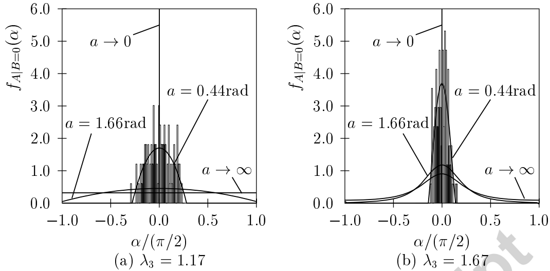
Figure 7: Conditional density function f_{A|B=0}(\alpha) for stretches (a) \lambda_3 = 1.17 and (b) \lambda_3 = 1.67 . Histogramical data from Walmsley and Murphy (1987) (bars) are shown together with model predictions (solid lines) for four values of the dispersion parameter a .
